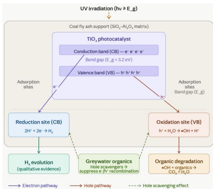
Figure 6. Proposed integrated photocatalytic mechanism of the TiO 2 –coal fly ash system: simultaneous oxidative organic degradation and reductive hydrogen evolution using laundry greywater as the reaction medium and hole scavenger.
