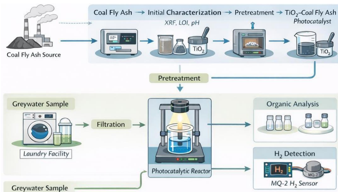
Figure 1. Schematic illustration of the experimental workflow for TiO 2 –coal fly ash photocatalytic treatment of greywater, including material characterization, pretreatment, photocatalytic operation, organic analysis, and qualitative hydrogen detection
