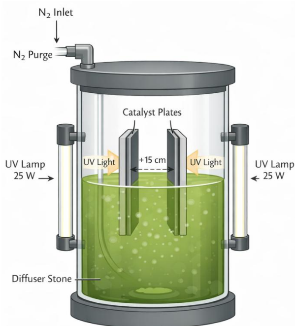
Figure 2. Schematic illustration of the closed borosilicate glass batch reactor used in the photocatalytic experiments, showing the configuration of two UVB lamps (25 W each) positioned on either side of the reactor at a distance of \pm 15 cm from the catalyst surface, the vertically installed \text{TiO}_2 -coal fly ash-coated stainless steel catalyst plates positioned at the center of the reactor, the nitrogen ( \text{N}_2 ) inlet and purge line at the top, and the diffuser stone at the base of the reactor.
