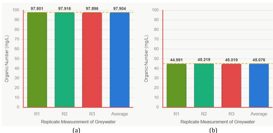
Figure 4. Organic content values (a) prior to and (b) following 6 hours of treatment in the integrated TiO 2 –coal fly ash/UV system
