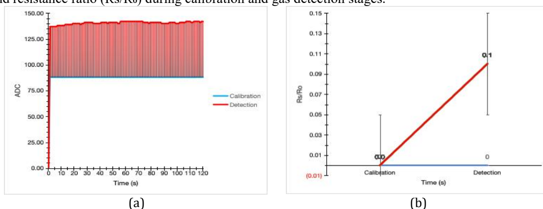
Figure 5. Qualitative response of MQ-2 sensor during reducing gas detection in the photocatalytic system: (a) sensor output response (ADC value) as a function of time during calibration and gas detection stages, and (b) comparison of R_s/R_0 ratio between baseline (calibration) and gas exposure conditions.
